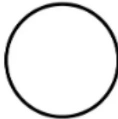
FIRST QUARTER
