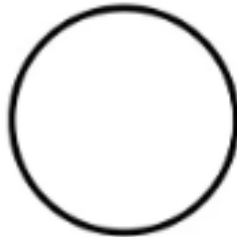
FULL MOON
