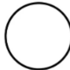
WANING CRESCENT
