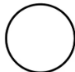
WANING GIBBOUS
