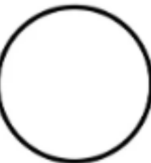
LAST QUARTER
